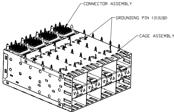
Z-8242410*0010* AS SHOWN WITH INNER & OUTER LIGHT PIPE 〈產品帶內外燈,帶抓板腳圖示〉
